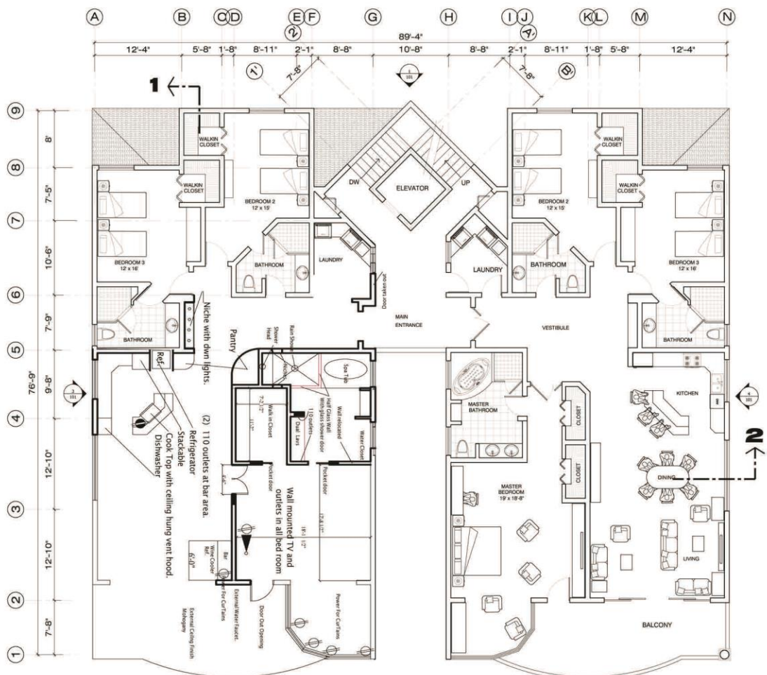
FURNITURE PLAN LAYOUT SECOND FLOOR
